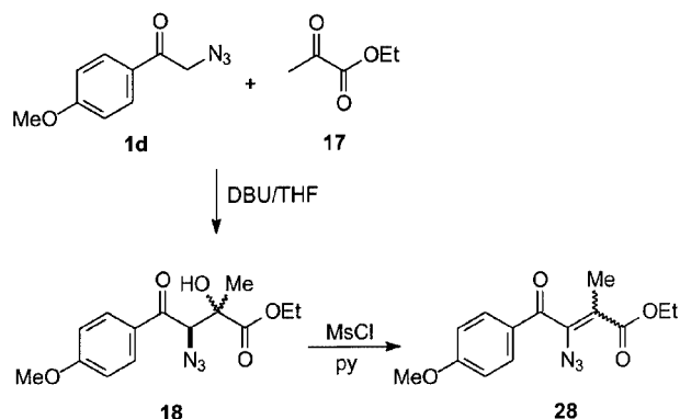
Scheme 3. Synthesis of \alpha -oxo ester 18 and its transformation into vinyl azide 28
