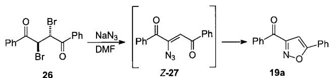
Scheme 5. Independent route to isoxazole 19a
