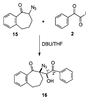
Scheme 2. Reaction between 2-azidobenzosuberone ( 15 ) and phenylglyoxal ( 2 )
