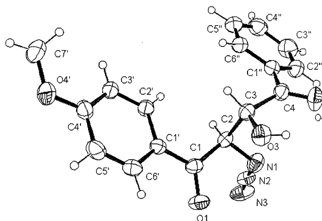
Figure 1. Crystal structure of azido alcohol syn - 6d
