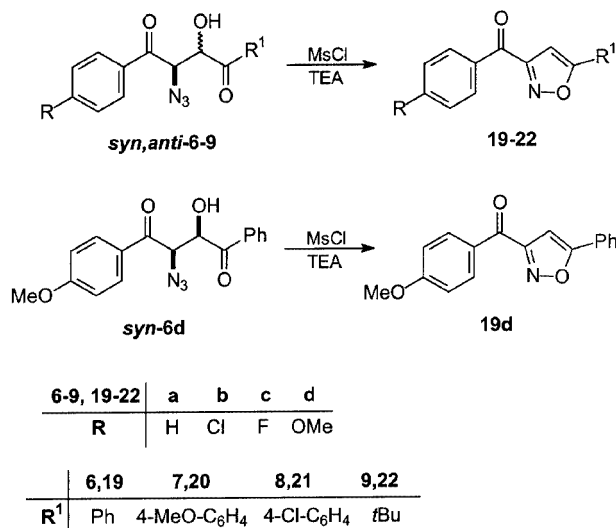
Scheme 4. Formation of isoxazoles 19–22 from azido alcohols 6–9
