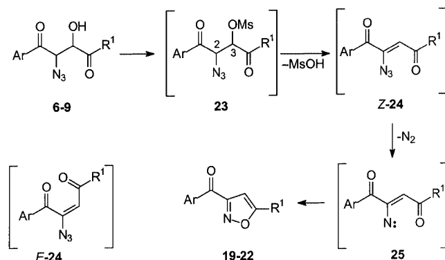
Scheme 6. Postulated intermediates in the formation of isoxazoles 19–22
