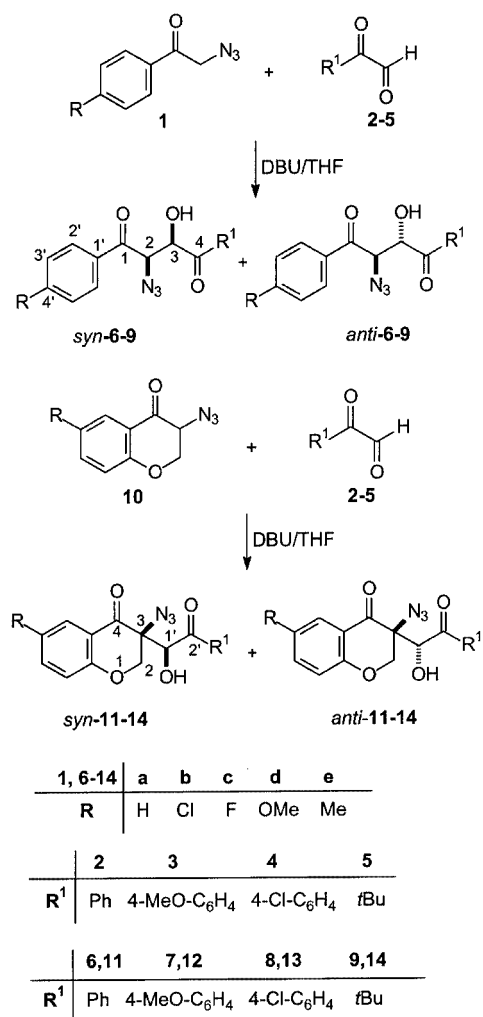
Scheme 1. Reactions between \alpha -azido ketones 1 and 10 and \alpha -oxo aldehydes 2–5
