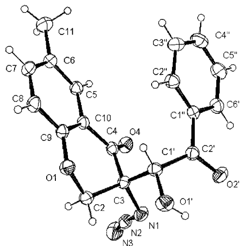
Figure 2. Crystal structure of azido alcohol anti - 11e
